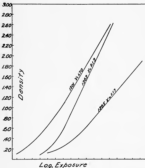
FIG. 2. Sensitometric curves of film stocks.
